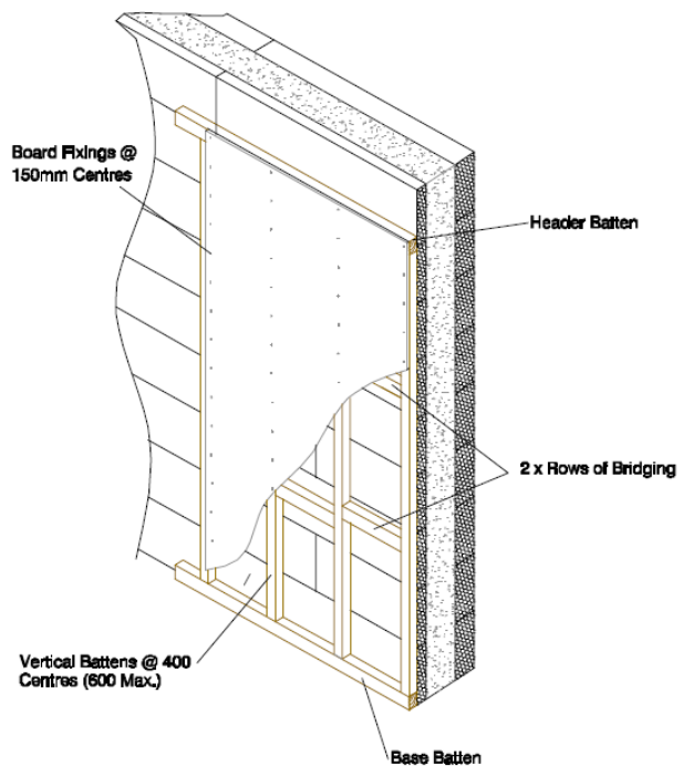
W29 - Wallboard fixed to Batten on Thermowall
