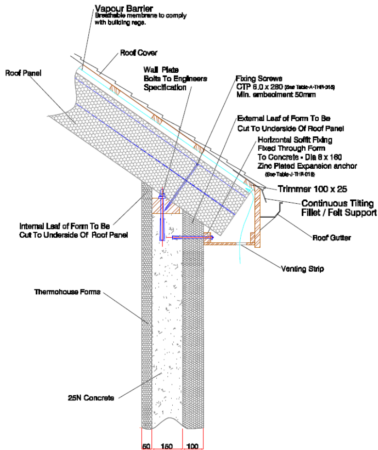
TR26 – Straight End Thermorooft Section Typical Detail
