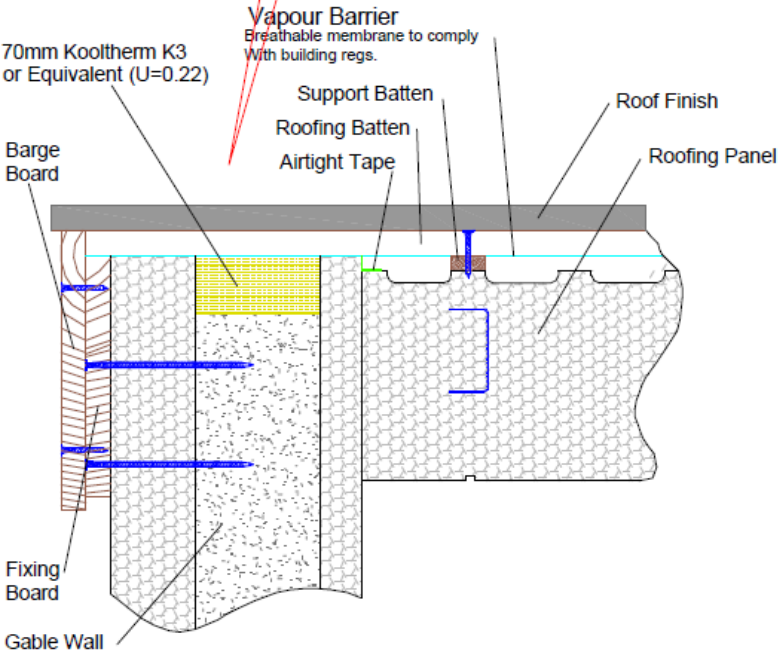
TR21 –Dormer Window Typical Detail
