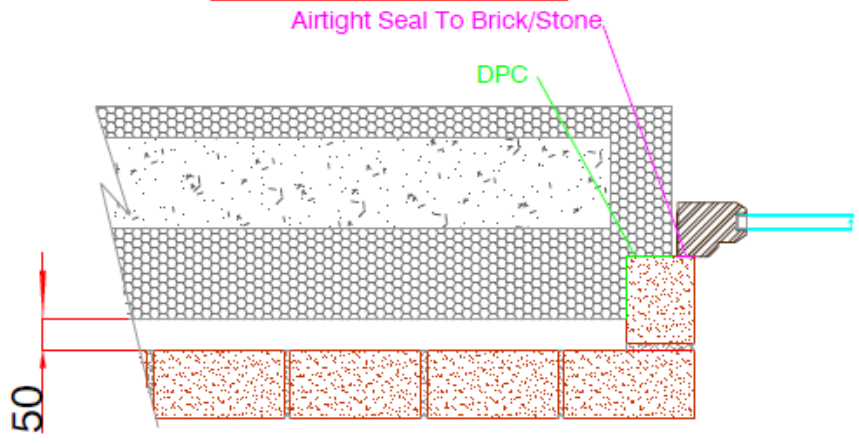
Section - Window Reveal
