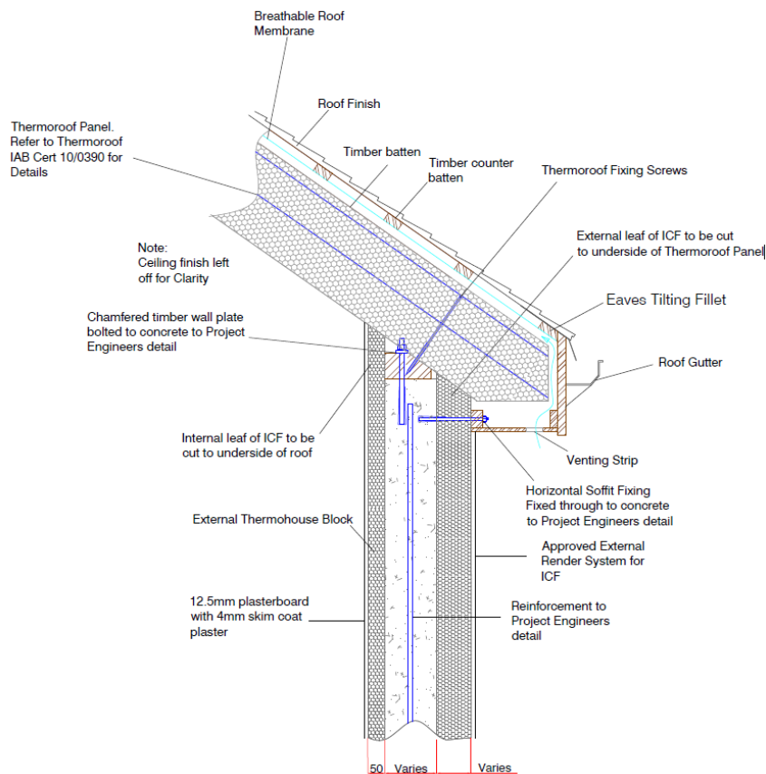
TR4 - ThermorooF to Thermowall Typical Detail
