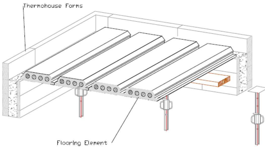
TF8 Step 1 – Place acrows and supports in place to place thermofloor over
