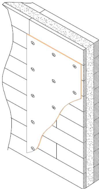
Board Fixings :- Plastic Insulated Anchors Installed to Manufacturers Recommendations
