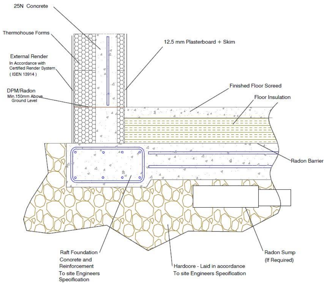
F4 Typical Raft Foundation Detail
